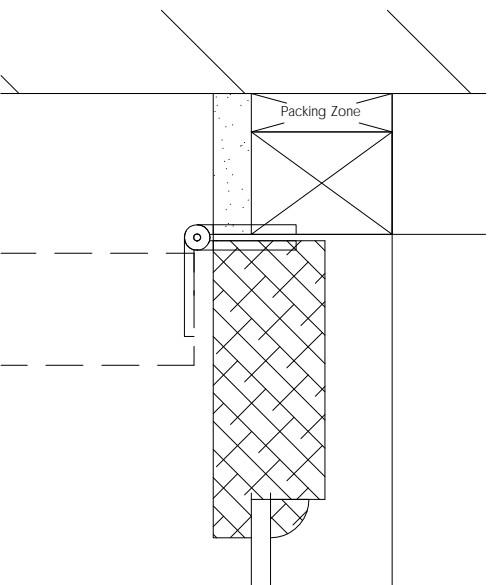
5 - Corner Detail At Wall
