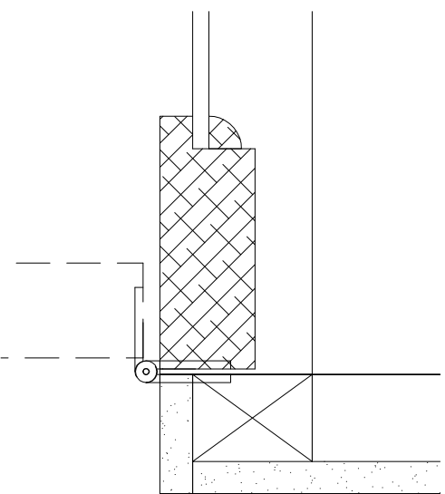
6 - Corner Detail
