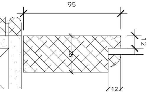
4 - Door Stile Detail
